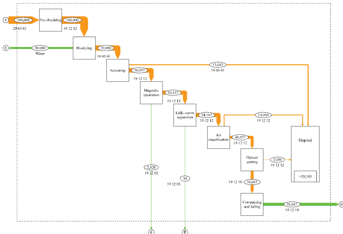
Figure 1 Material flow of residual waste in the mechanical-biological treatment plant at the WMC Mariščina, Croatia; I – import flow; E – export flow
