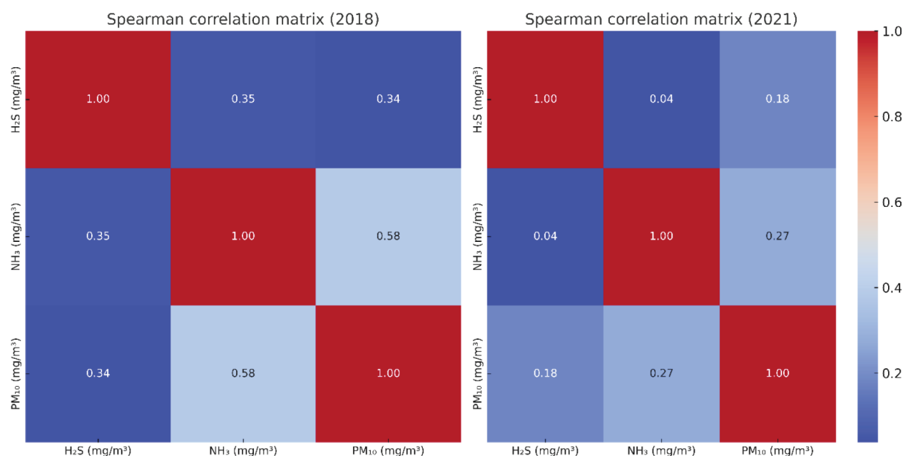
Figure 9 Spearman's rank correlation matrix illustrating the relationships between \text{H}_2\text{S} , \text{NH}_3 , and \text{PM}_{10} levels measured in ambient air near the WMC Mariščina for the years 2018 and 2021. The colour scale represents the strength and direction of the correlations, with values ranging from -1 (perfect negative correlation) to 1 (perfect positive correlation)
