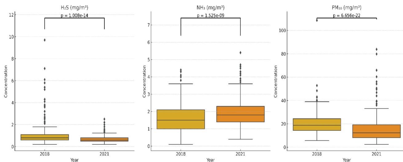
Figure 7 Comparison of 2018 and 2021 H_2S , NH_3 , and PM_{10} levels measured near the WMC Mariščina. The central line within each box represents medians, while the edges of the box indicate the interquartile range (IQR). Whiskers extend to the minimum and maximum values within 1.5 times of the IQR, and any outliers are plotted as individual points
