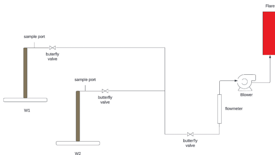
Figure 2 Active venting system schematic at the HDPE cover WMC Mariščina landfill. W1 – gas well 1; W2 – gas well 2
