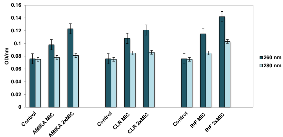
Figure 2. Leakage of nucleic acids (260 nm) and proteins (280 nm) from M. intracellulare after application of selected antimicrobial drugs at MIC and 2 × MIC (MIC—minimum inhibitory concentration; AMIKA—amikacin; CLR—clarithromycin; RIF—rifampicin). The experiment was repeated three times in duplicate and the mean value ± SD is shown.
