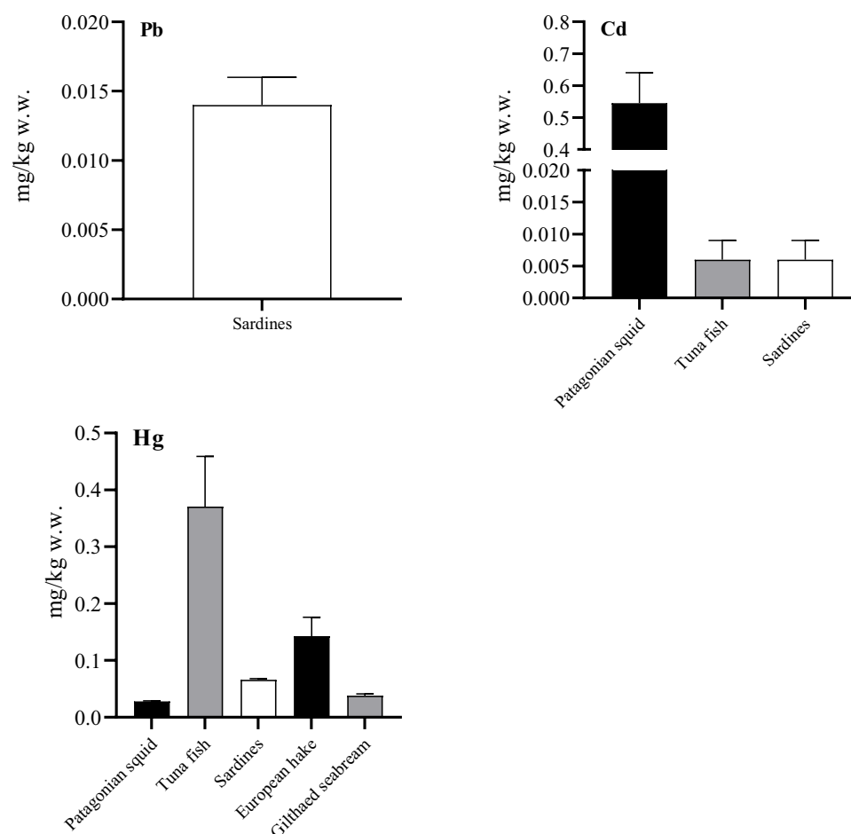
Figure 2. Comparison of heavy metal concentrations (Pb, Cd, Hg) between the tested species.
