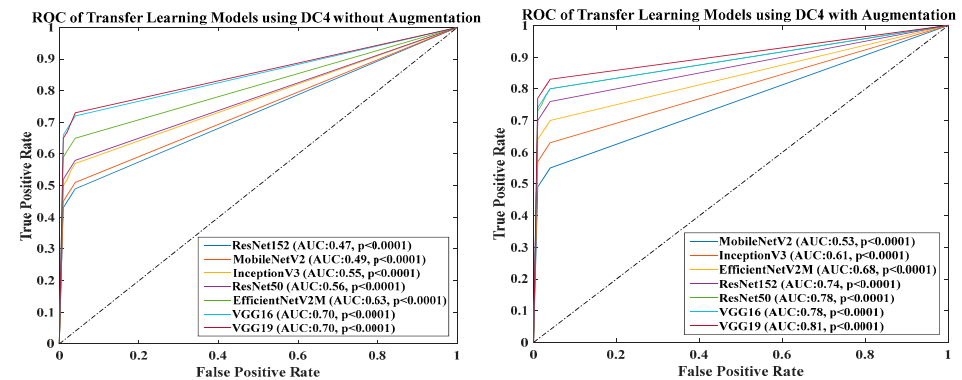
Figure 27. ROC of seven TLs using DC4 with augmentation and without augmentation.
