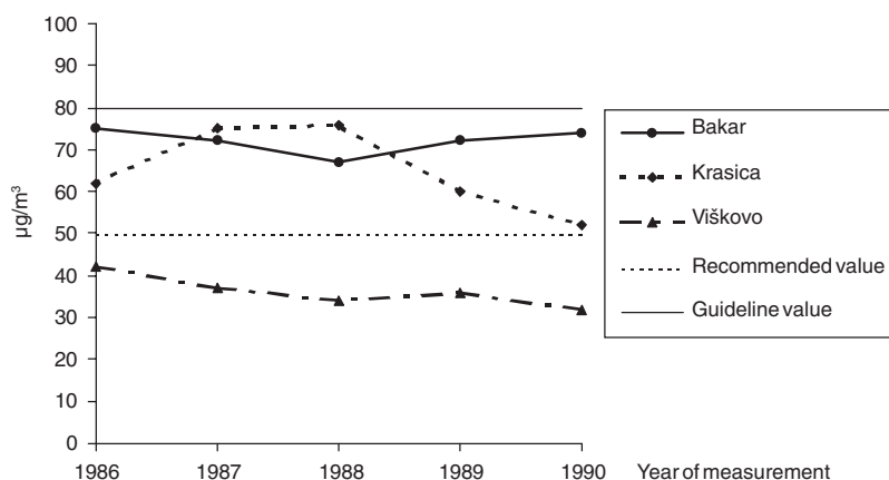
Figure 1 Mean annual SO 2 concentrations for the period 1986–1990
