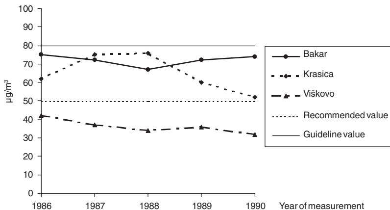
Figure 1 Mean annual SO 2 concentrations for the period 1986–1990
