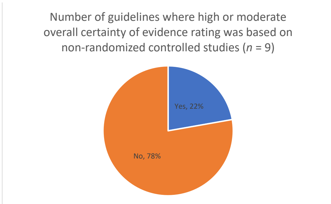
Figure 4. Moderate or high certainty of evidence rating based on non-randomized studies.
