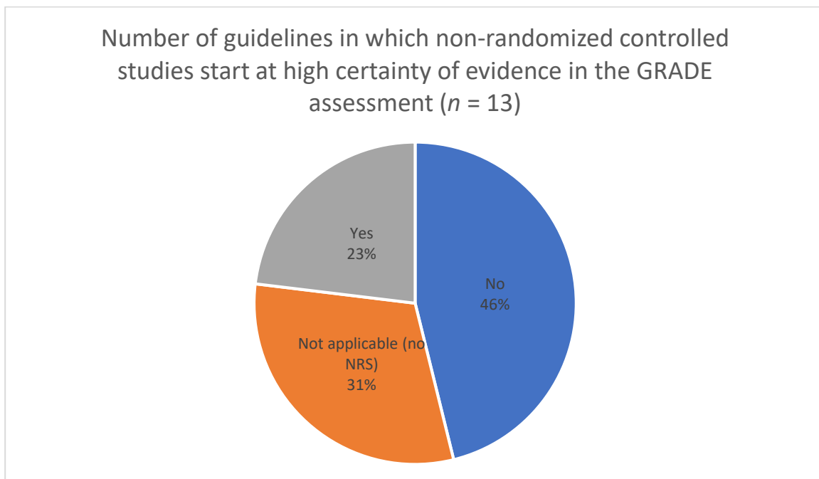
Figure 5. Certainty of evidence assessment for NRS—initial rating at high.
