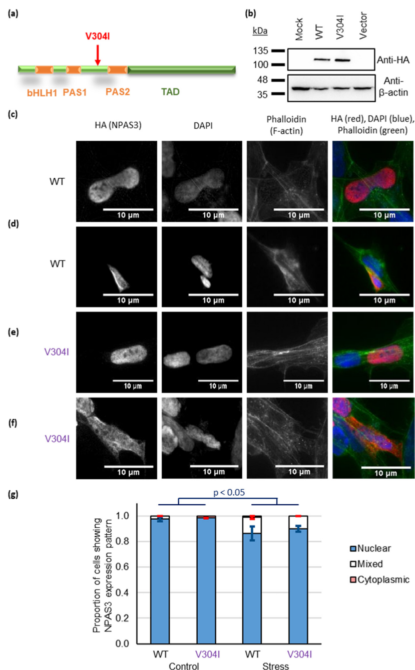
Figure 2. Mislocalization of NPAS3 to the cytoplasm does not require the V304I mutation, as determined in SH-SY5Y neuroblastoma cells. (a) One-dimensional schematic of the NPAS3 protein, showing major domains and the location of the V304I mutation. Abbreviations: bHLH: Basic helix-loop-helix domain, PAS: Per-Amt-Sim domain, TAD: C-terminal activator domain. (b) Expression of NPAS3 wild type (WT) and V304I mutant constructs, confirmed by Western blotting in HEK293 cells. Negative controls are mock transfection and transfection with empty vector only, (c–f) Typical localization patterns of NPAS3, both wild type and mutant V304I when over-expressed in SH-SY5Y cells, with each showing a mixture of nuclear and cytoplasmic localization: (c) WT in the nucleus, (d) WT in the nucleus and cytoplasm, (e) V304I in the nucleus, (f) V304I in the cytoplasm. The nucleus (DAPI) and actin cytoskeleton (phalloidin) are shown for context. (g) Quantification of the localization patterns from parts c–f in a blinded experiment. Cells were transfected with either WT or V304I NPAS3 and then exposed to either sodium arsenite (which induces oxidative stress) or an equivalent volume of DMSO as a control. 8 experimental replicates were performed for each combination of plasmid/stress status, with 7–10 cells being counted in each replicate.
