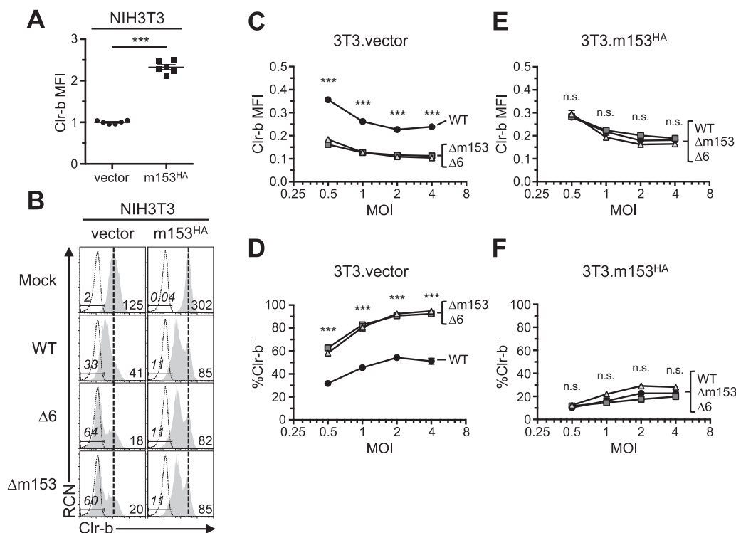
FIG 7 Complementation of m153 abrogates Clr-b loss observed in m153-deficient virus. NIH 3T3 cells were transfected with pTRIPZ lentivirus expressing m153 or empty vector and infected with MCMV. (A) Comparison of the Clr-b expression on resting transfected cells. (B) Histograms of Clr-b levels on NIH 3T3.vector and NIH 3T3.m153 HA fibroblasts upon infection with MCMV (WT, Δ6, or Δm153). (C and D) Analysis of NIH 3T3.vector cells by quantitation of Clr-b MFI (C) and quantitation of percent Clr-b - cells at different MOI (D). (E and F) Analysis of NIH 3T3.m153 HA cells by quantitation of Clr-b MFI (E) and quantitation of percent Clr-b - cells at different MOI (F). Data were analyzed using 2-way ANOVA and are representative of those from 3 independent experiments.
