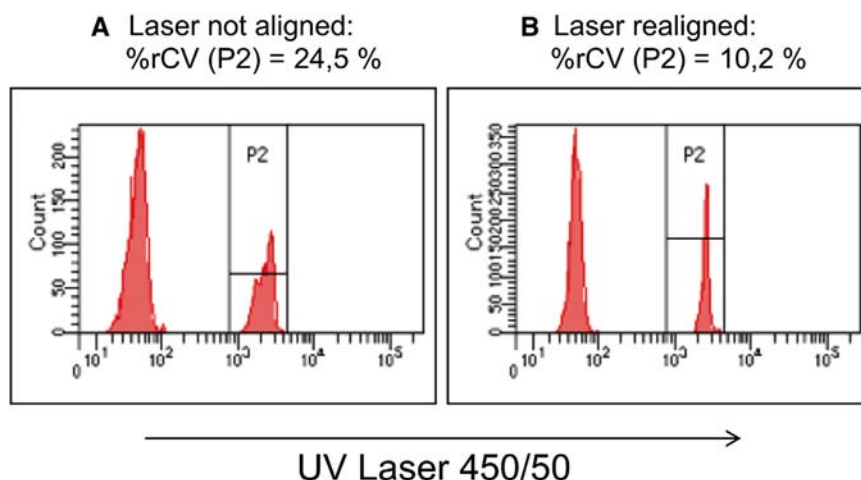
Figure 11. How one can detect suboptimal alignment of lasers. Both histograms display a negative and positive bead population in the 450/50 channel of the UV-Laser of a BD FAC-SCaria SORP cell sorter. Although the positive peak in (A) still falls into the defined target area (brackets = P2), the shape and %CV of the peak suggest a suboptimal alignment of the UV-Laser. After realignment the shape of the positive peak become narrower with only the half of the %CV. (B) Laser-alignment is optimal, when the lowest %CV values are reached.
