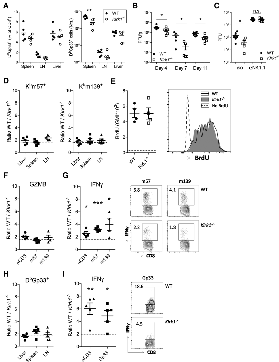
Figure 4. NKG2D deficiency impairs IFN- \gamma production but not proliferation of mCMV-specific CD8 ^{+} T cells. (A) WT and Klrk1 ^{-/-} mice were infected with LCMV. After 8 days, the percentage and absolute number of antigen-specific CD8 ^{+} T cells was determined in spleen, inguinal LNs, and liver. (B) WT and Klrk1 ^{-/-} mice were infected with mCMV and kinetics of viral load was followed over time in the liver. (C) Mice were treated with isotype or NK-cell depleting antibodies. After 1 day, mice were infected with mCMV. Four days after infection, virus titers were determined in spleen. (D) mBMCs (WT: Klrk1 ^{-/-} , 1:1) were infected with mCMV and after 8 days, ratios between WT and Klrk1 ^{-/-} cells were determined within K ^{b} m57 ^{+} and K ^{b} m139 ^{+} effector cells. Dashed lines indicate CD8 ^{+} T-cell ratio in blood before infection. (E) mBMCs were infected with mCMV. On days 1, 3, 5, and 7 after infection, mice were injected with BrdU. On day 8 after infection, BrdU labeling of effector CD8 ^{+} T cells was determined in blood. Dashed line indicates BrdU staining of CD8 ^{+} T cells from animals that were not injected with BrdU. (F and G) mBMCs were infected with mCMV. On day 8 after infection, the ratio within (F) granzyme B (GZMB) and (G) IFN- \gamma -producing cells after in vitro restimulation of splenic T cells with anti-CD3 \epsilon antibodies or with m57 or m139 peptides. FACS plots are gated for CD8 ^{+} cells. (H–I) mBMCs (WT: Klrk1 ^{-/-} , 1:1) were infected with LCMV and after 8 days, ratios between WT and Klrk1 ^{-/-} cells were determined in spleen. Dashed lines indicate CD8 ^{+} T-cell ratio in blood before infection. (H) Ratio within K ^{b} Gp33 ^{+} effector cells. (I) Ratio within IFN- \gamma -producing cells after in vitro restimulation with anti-CD3 \epsilon antibodies or Gp33 peptides. FACS plots are gated for CD8 ^{+} cells. Data shows mean \pm SEM and are representative of two (A–C, E, H–I), or four (D, F) experiments with four to five mice per experiment. * p < 0.05 , ** p < 0.005 , *** p < 0.001 (Student's t-test or ANOVA with Bonferroni's post-test).
