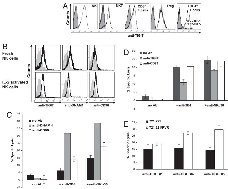
Fig. 4. TIGIT function on primary immune cells. (A) TIGIT is expressed by NK, NKT, Treg, CD8 + T cells and memory CD4 + T cells. FACS analysis of freshly isolated peripheral blood lymphocytes subsets (indicated in the histograms) stained for TIGIT expression. NK cells were characterized by CD3 + CD56 + , NKT cells by CD3 + CD56 + , T cells either by CD8 + CD56 - or by CD4 + CD56 - , Treg cells are CD4 + CD25 + FOXP3 + and memory CD4 + T cells were characterized by CD45RO staining (right histogram). (B) Flow cytometry of freshly isolated or IL-2-activated NK cells stained for TIGIT, DNAM1, and CD96 expression. Gray shaded histograms, background staining with the secondary fluorescein-conjugated antibody only. (C) DNAM1 and CD96 are costimulatory receptors. P815 cells were incubated either with no mAb or with the combinations of anti-2B4 or anti-NKp30 mAbs (indicated in the x axis) and anti-DNAM1 or with anti-CD96 mAb (indicated by the different column colors). Redirected NK cytotoxicity against P815 cells was determined at E:T ratio of 3:1. (D) P815 cells were incubated either with no mAb or with combinations of anti-2B4 or anti-NKp30 mAbs (indicated in the x axis) with and without anti-TIGIT, or with anti-CD99 (indicated by the different column colors) to redirect NK cytotoxicity. Effector IL-2 activated bulk NK cells were then added in E:T ratio of 5:1. The two redirected killing assays presented in C and D were done independently. (E) Killing of the target cells 721.221 and 721.221/PVR by primary NK cells at E:T ratio of 5:1. NK cells were preincubated with the various mAb indicated in the x axis.
