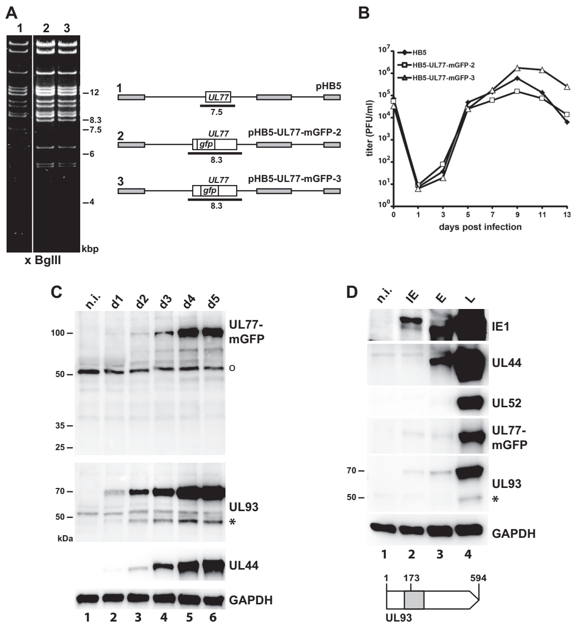
FIG 1 Characteristics of HCMV mutants expressing a UL77-mGFP fusion protein. (A) Construction of the recombinant HCMV BACs pH5-UL77-mGFP-2 and pH5-UL77-mGFP-3, which differ in the position of the mGFP sequence inserted into the UL77 open reading frame (ORF). The schematic drawing of the respective BACs is given to the right (pHB5, parental genome), with the expected BglII restriction fragments indicated as black lines. Gray boxes represent repeat regions of the HCMV genome. The left part shows the BglII restriction pattern of the parental BAC (lane 1) compared to that of the mutant genomes (lanes 2 and 3). (Please note the shift of a 7.5-kbp fragment in pH5 to 8.3 kbp in the UL77-mGFP mutants.) (B) Growth kinetics of the parental virus HB5 (black diamonds) and the HCMV mutants expressing the UL77-mGFP fusion proteins (open triangles and squares, respectively). Fibroblasts were infected at a multiplicity of infection (MOI) of 0.1, supernatants were taken at the time points indicated postinfection, and titers were determined by plaque assay. The values for time point 0 indicate the inoculation doses. (C) Expression of the UL77-mGFP fusion protein and the UL93 protein after infection of fibroblasts with HB5-UL77-mGFP-3 (MOI of 1). Cell lysates were prepared on days 1 to 5 p.i. and analyzed for the indicated proteins by immunoblotting. pUL77-mGFP was detected with a GFP-specific antibody. The nonspecific reactivity with a cellular protein is marked with an open circle. The HCMV early protein pUL44 served as control for viral gene expression and GAPDH as a loading control. Molecular mass markers (in kildodaltons) are given to the left. n.i., noninfected fibroblasts. The asterisk denotes the putative 48-kDa version of pUL93. (D) Expression kinetics of the UL77-mGFP and UL93 proteins. IE, immediate early (i.e., treatment with cycloheximide/actinomycin D); E, early (i.e., treatment with phosphonoacetic acid); L, late (i.e., protein expression in the absence of inhibitors). Fibroblasts were infected with HB5-UL77-mGFP-3 at an MOI of 1, kept with or without the respective inhibitors, followed by preparation of cell lysates on day 3 p.i. and analysis by immunoblotting. IE1, UL44, and UL52 are representative IE, E, and L viral proteins. The open arrow depicts the full-length UL93 ORFs (codons 1 to 594). A putative internal initiation codon at position 173 would give rise to the synthesis of a 48-kDa protein. The part of the UL93 ORF marked in gray was used to express a recombinant protein employed for generation of the specific antibody.
