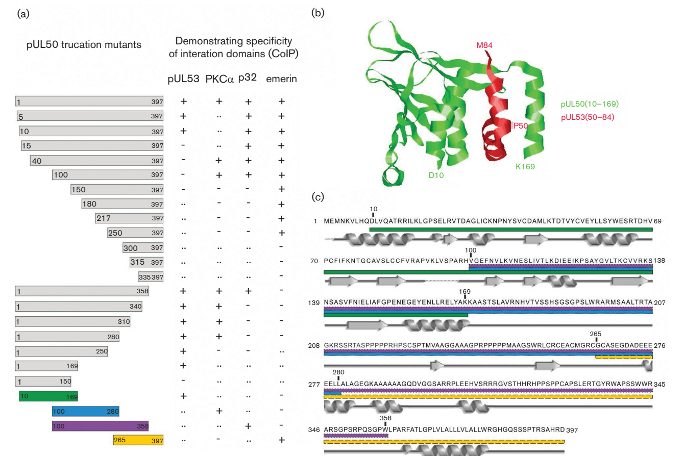
Fig. 5. Regions and secondary structural elements determining binding properties of pUL50. (a) Schematic presentation of ColIP data obtained with N- and C-terminal truncation mutants of pUL50 (this study and Milbradt et al. , 2009, 2012, 2014). Note, specific regions of pUL50 responsible for interaction with pUL53 (green), PKC \alpha (blue), p32 (purple) and emerin (yellow). +, ColIP positive; -, ColIP negative; .., not determined. (b) Ribbon presentation of the reciprocal interaction domains comprised in the recently solved crystal structure of the pUL50-pUL53 core NEC (PDB code 5D5N; Walzer et al. , 2015): pUL53 interaction domain within pUL50 (amino acids 10-169) depicted in green, pUL50 interaction domain within pUL53 (amino acids 50-84) (Sam et al. , 2009) depicted in red. (c) Schematic presentation of the pUL50 secondary structure. Secondary structure prediction of amino acids 172-397 was performed with the JPred 4 ( http://www.compbio.dundee.ac.uk/jpred/ ) prediction tool. Secondary structural elements contained within amino acids 1-171 are derived from the crystal structure (b). Identified interaction domains within pUL50 are highlighted by shaded boxes (green, pUL53; blue, PKC \alpha ; purple, p32; yellow, emerin).
