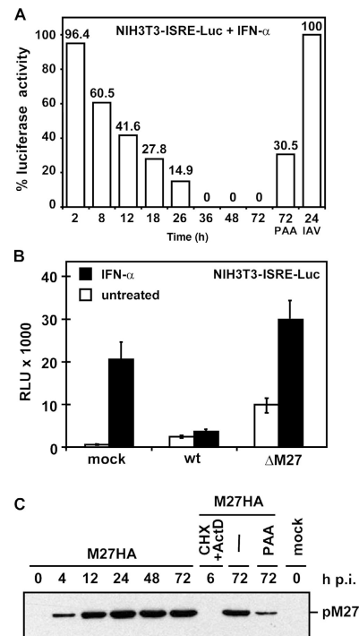
Figure 1. Inhibition of IFN- \alpha -dependent luciferase induction by MCMV M27 . (A) 3T3-ISRE-luc cells were infected with 10 PFU/cell MCMV-WT strain Smith and stimulated with 500 U/ml IFN- \alpha for 5 h at the indicated time points p.i. Results were expressed as the percentage of luciferase activity in comparison with uninfected cells. The influence of viral gene expression was studied by the analysis of luciferase activity in the presence of PAA, which inhibits the expression of viral late gene expression, and by the analysis of UV-inactivated virus (IAV). (B) 3T3-ISRE-luc cells were infected with MCMV-WT, \Delta M27-MCMV, or M27rev (10 PFU/cell each) and stimulated with 500 U/ml IFN- \alpha for 5 h at 8 h (mock) or 29 h (MCMV-WT and \Delta M27-MCMV) p.i. Luciferase activity was determined luminometrically as relative light units (RLU). Each value represents the mean \pm SD from three independent experiments. (C) Expression kinetics of the M27 protein. MEFs were infected with 10 PFU/cell M27HA, and cell lysates were prepared at the indicated time points. Equivalent amounts of lysate were subjected to SDS-PAGE and then immunoblotted using anti-HA antibodies. The selective synthesis of MCMV IE proteins was achieved by infecting cells in the presence of 50 \mu g/ml of cycloheximide, which was then replaced by 5 \mu g/ml of actinomycin for a further 2 h. 250 \mu g/ml PAA was used to inhibit late phase gene expression.
