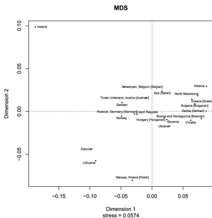
Figure 3. Multidimensional Scaling (MDS) plot showing genetic similarities between different SEE countries based on Y chromosome [39].
