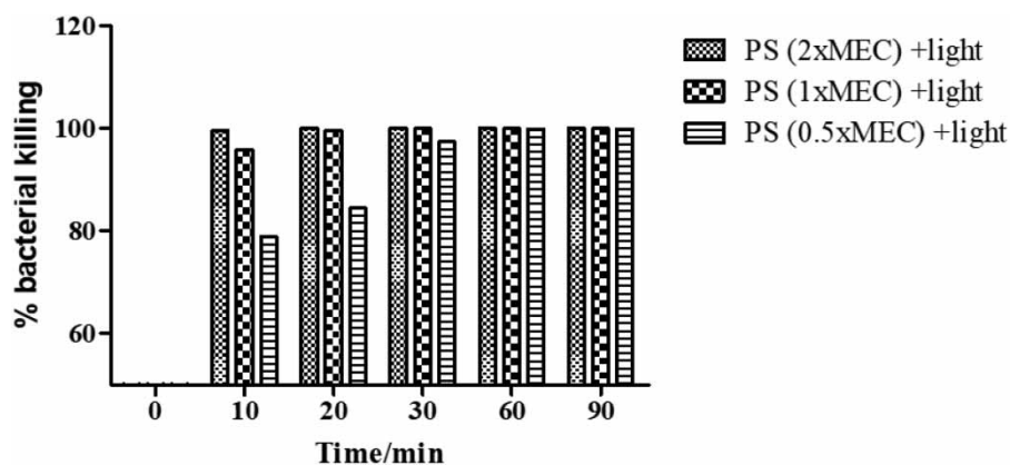
Figure 3 | Percentage of bacterial killing after photoinactivation with PS with and without light. L. pneumophila cells were incubated with PS in the dark and then treated for 10 min with a total dose of 12 \text{ J cm}^{-2} violet light or without light. Data are the mean of three independent experiments.
