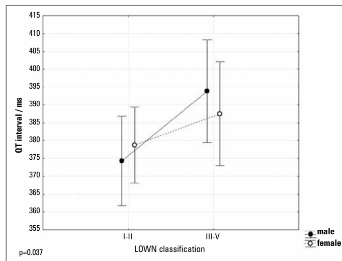
Figure 3. QT interval in patients with simple ( n=112 ) and complex VA ( N=75 ). Presented are mean values with 95% confidence intervals
