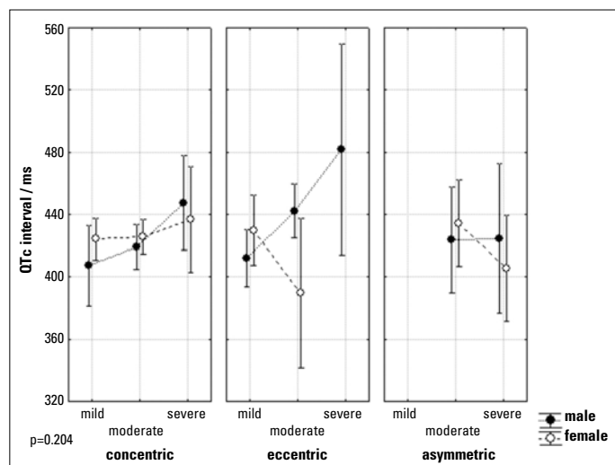
Figure 1. QTc interval in patients according to the type and degree of left ventricular hypertrophy. Presented are mean values with 95% confidence intervals
