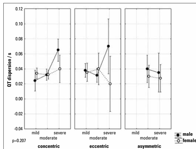
Figure 2. QT dispersion in patients according to the type and degree of left ventricular hypertrophy. Presented are mean values with 95% confidence intervals
