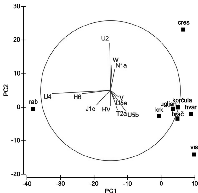
Fig. 3. PCA plot based on frequencies of subhaplogroups in analyzed island populations. The first 2 principal components describe 73.4% of variation.
